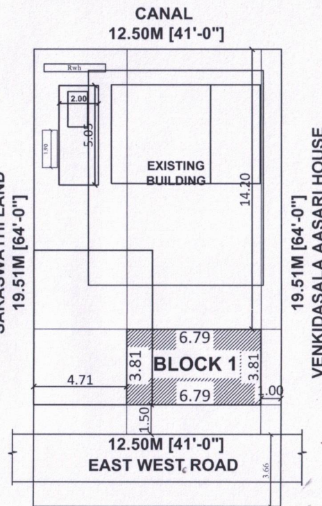
SITE PLAN
