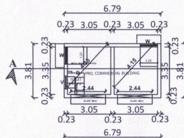
PRO. GROUND FLOOR
