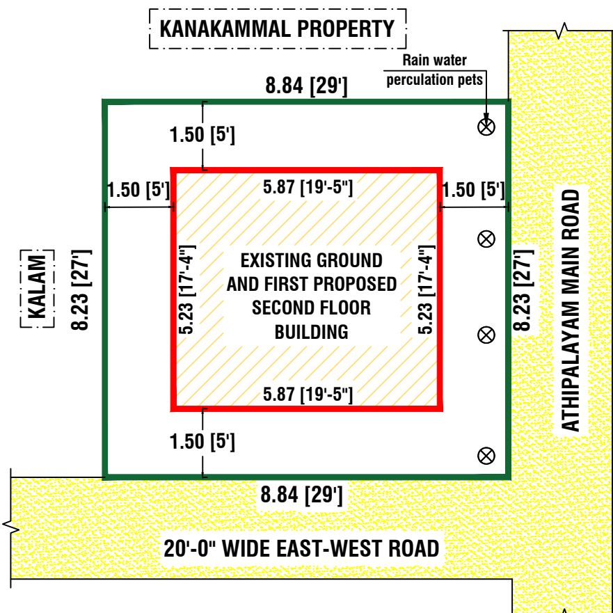
SITE PLAN
