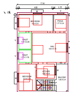
PROPOSED FIRST FLOOR BUILDING
