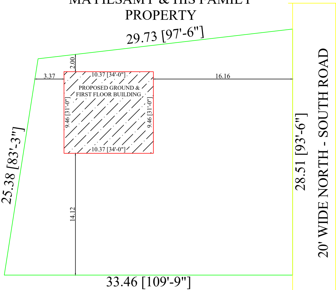
MAYILSAMY & HIS FAMILY PROPERTY SITE PLAN
