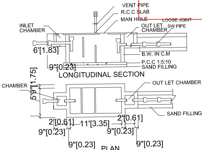
SEPTIC TANK:
