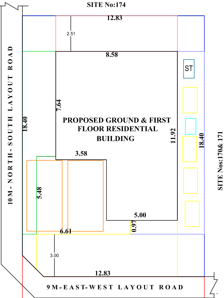
SITE PLAN
