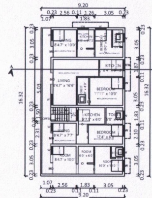
PROPOSED SECOND FLOOR
