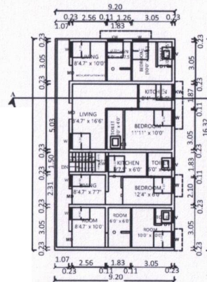
PROPOSED FIRST FLOOR
