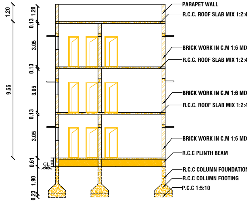
CROSS SECTION AT A-A
