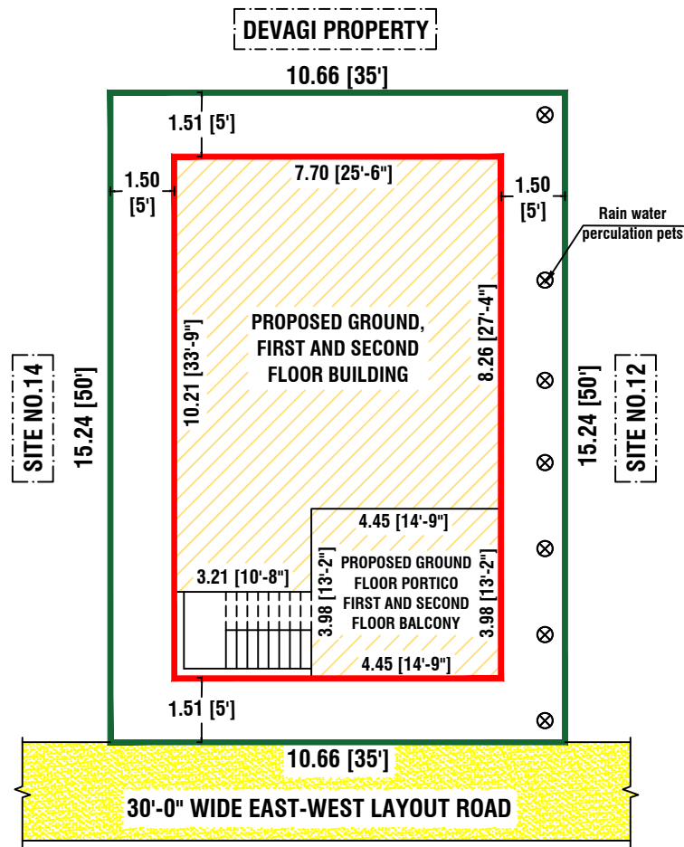
SITE PLAN
