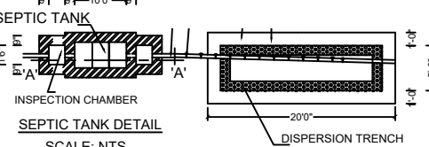
SEPTIC TANK DETAIL SCALE: NTS
