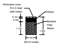
RAIN WATER HARVESTING RECHARGE TRENCH SECTION
