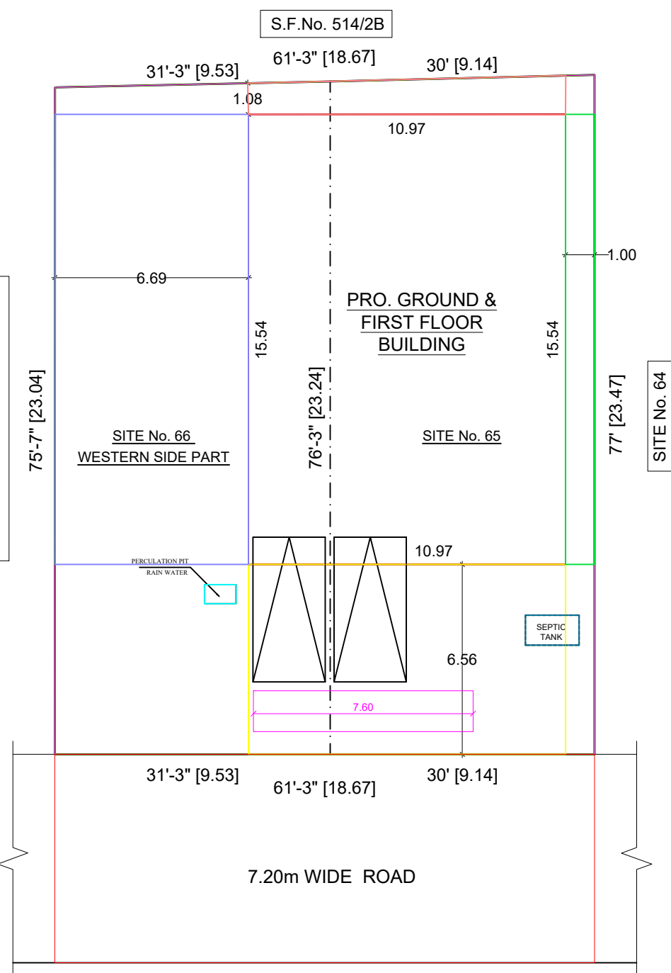
SITE PLAN
