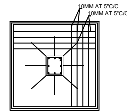
FOOTING DETAIL SCALE: NTS
