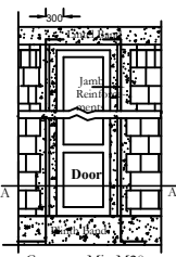
Sectional Elevation of Door
