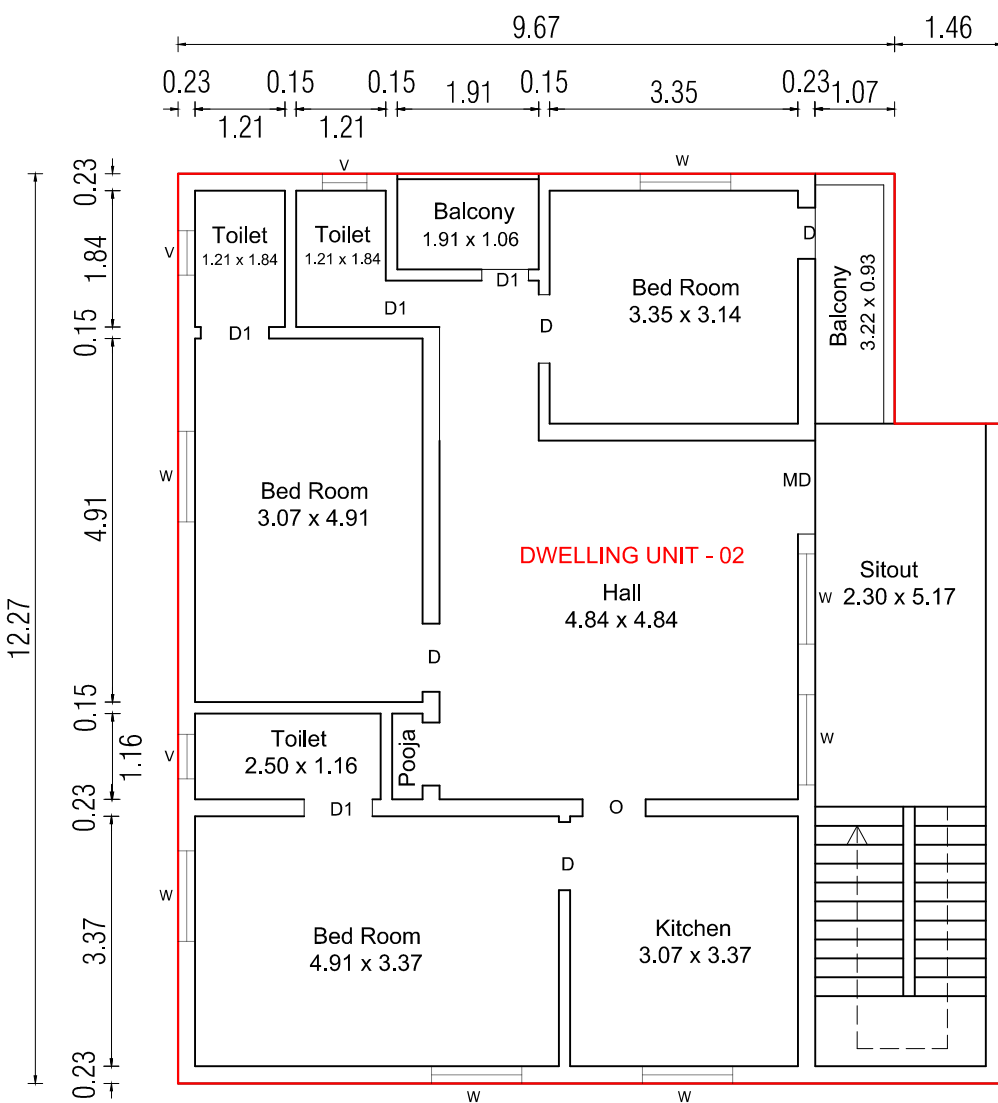
FIRST FLOOR PLAN (PROPOSED FIRST FLOOR)
