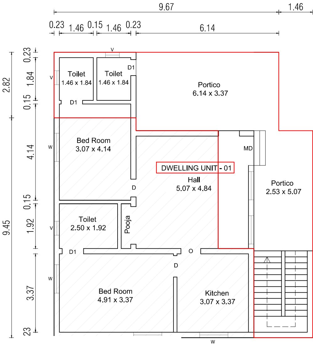
GROUND FLOOR PLAN (EXISTING BUILDING)
