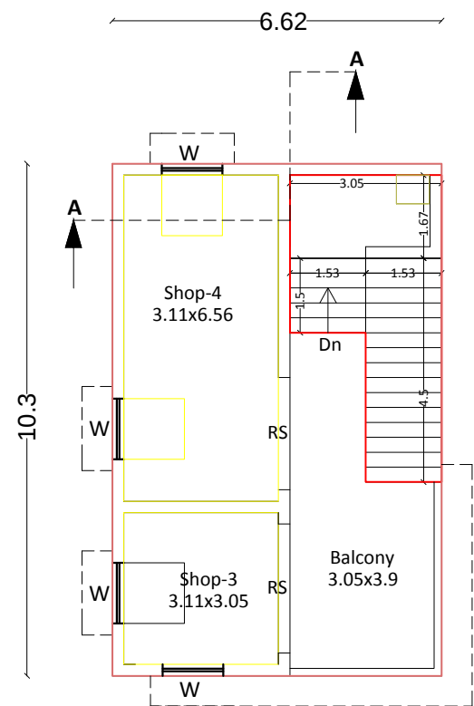
PRO.FF PLAN
