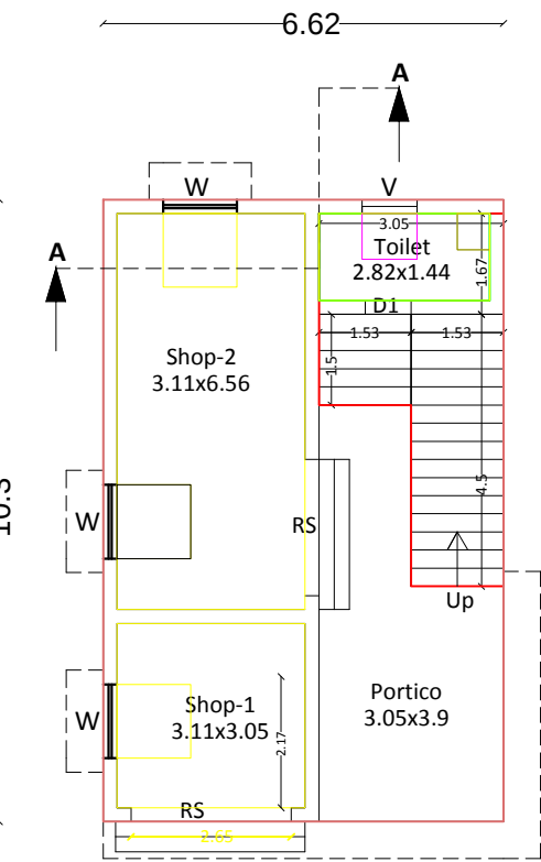
PRO.GF PLAN
