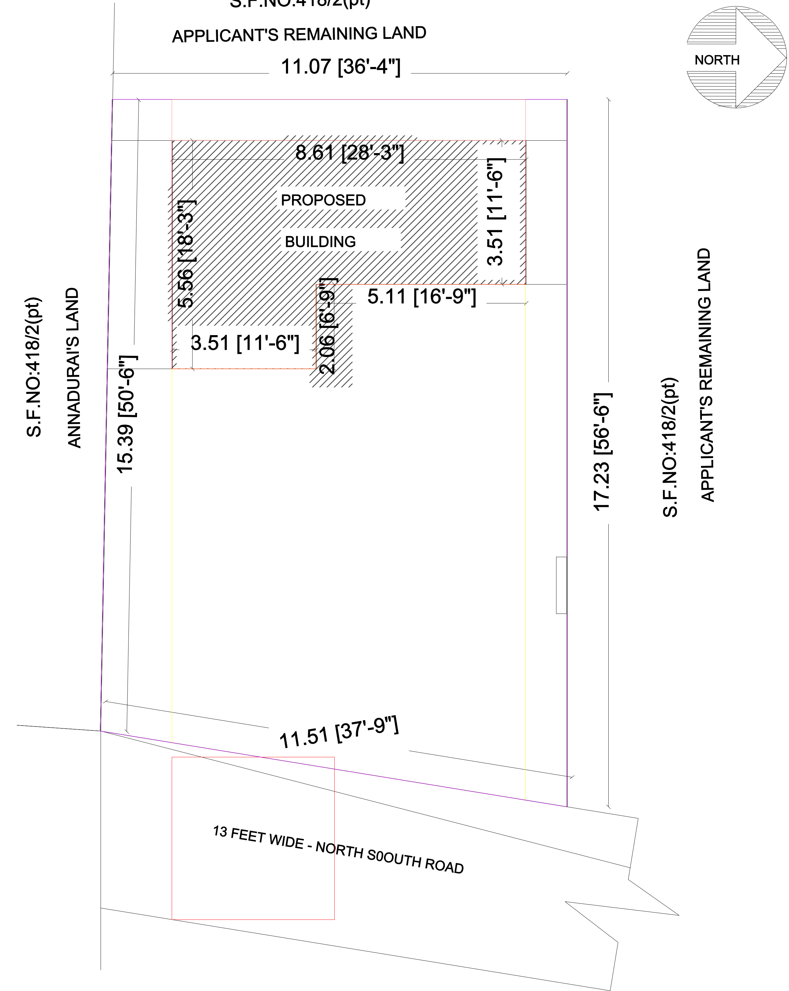
SUPER IMPOSED PLAN (AREA TAKEN FOR CONSTRUCTION) (SCALE:1=100)
