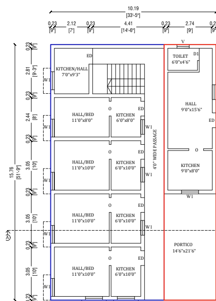
EXI. GF &F.F AND ADDITIONAL PROPOSED GF & FF PLAN
