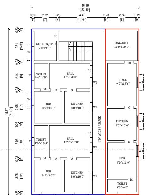
EXI. GF & F.F AND ADDITIONAL PROPOSED GF & FF PLAN
