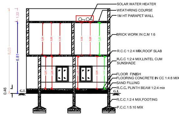
SECTION AT ( B - B )
