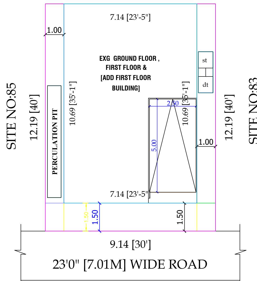
SITE PLAN
