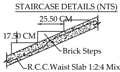
STAIRCASE DETAILS (NTS)
