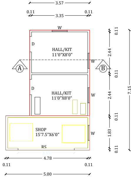
ADD.GROUND FLOOR PLAN
