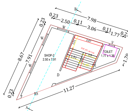
PRO.FIRST FLOOR PLAN
