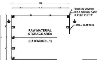
PLAN SCALE : 1" = 8' 0"
