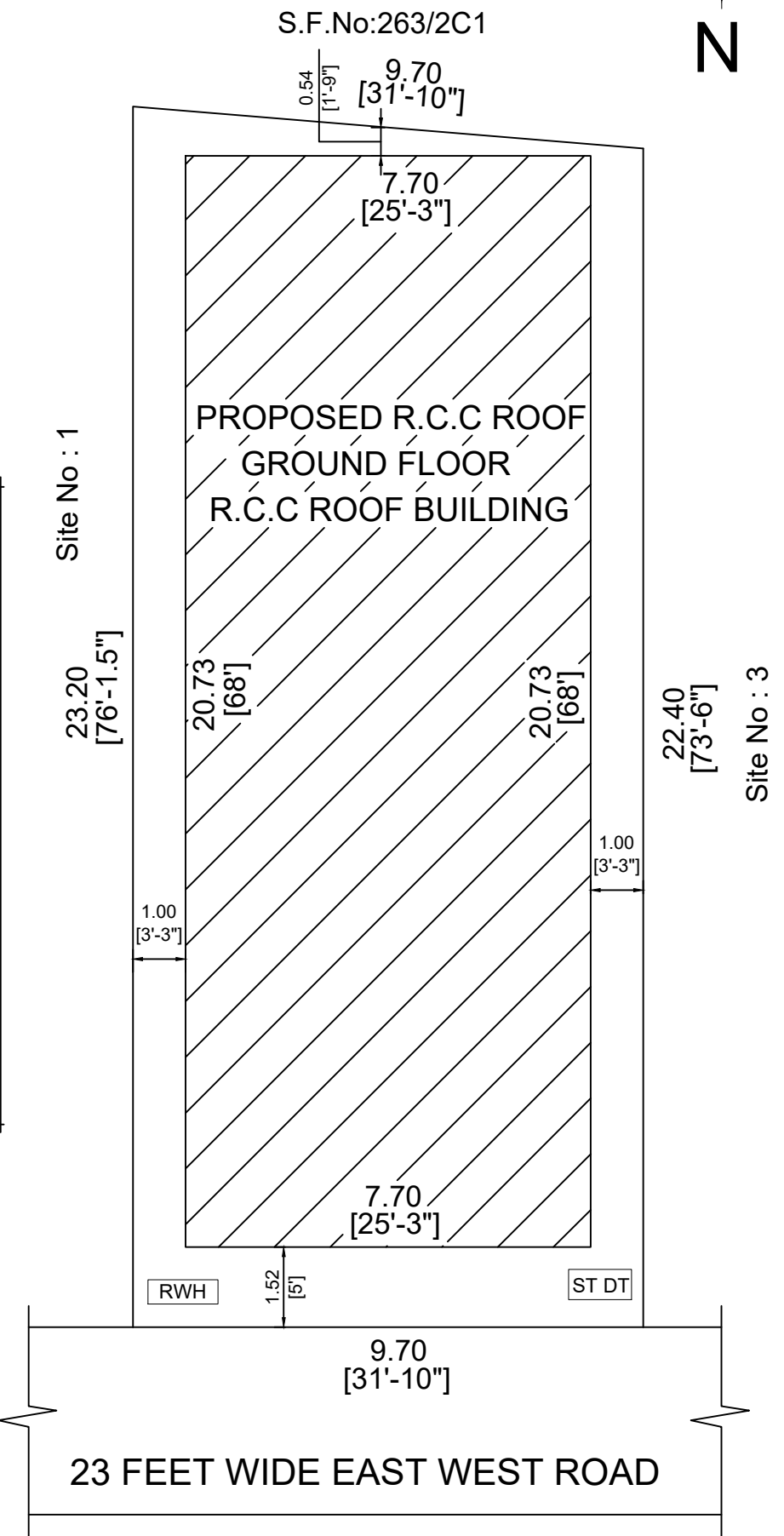
SITE PLAN
