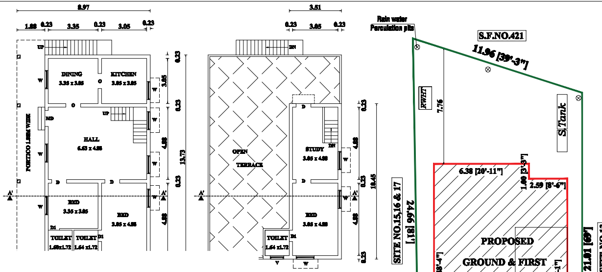
FLOOR PLAN
