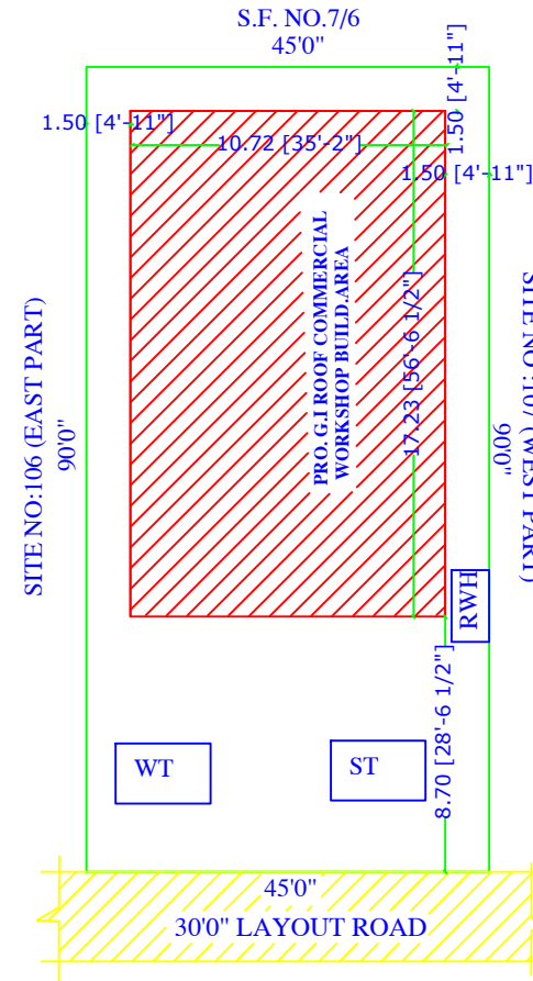
SITE PLAN
