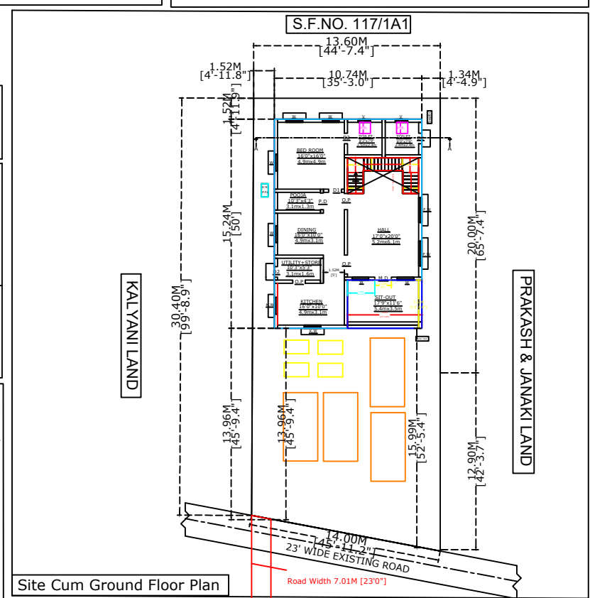
Site Cum Ground Floor Plan
