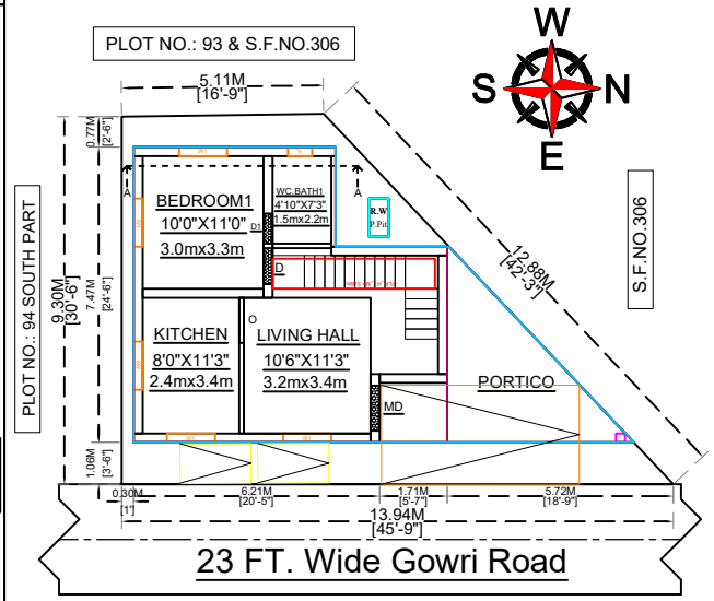
SITE CUM PROPOSED GROUND FLOOR PLAN
