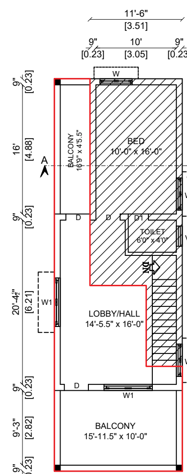
EXI. & PRO. ADDL. FIRST FLOOR PLAN
