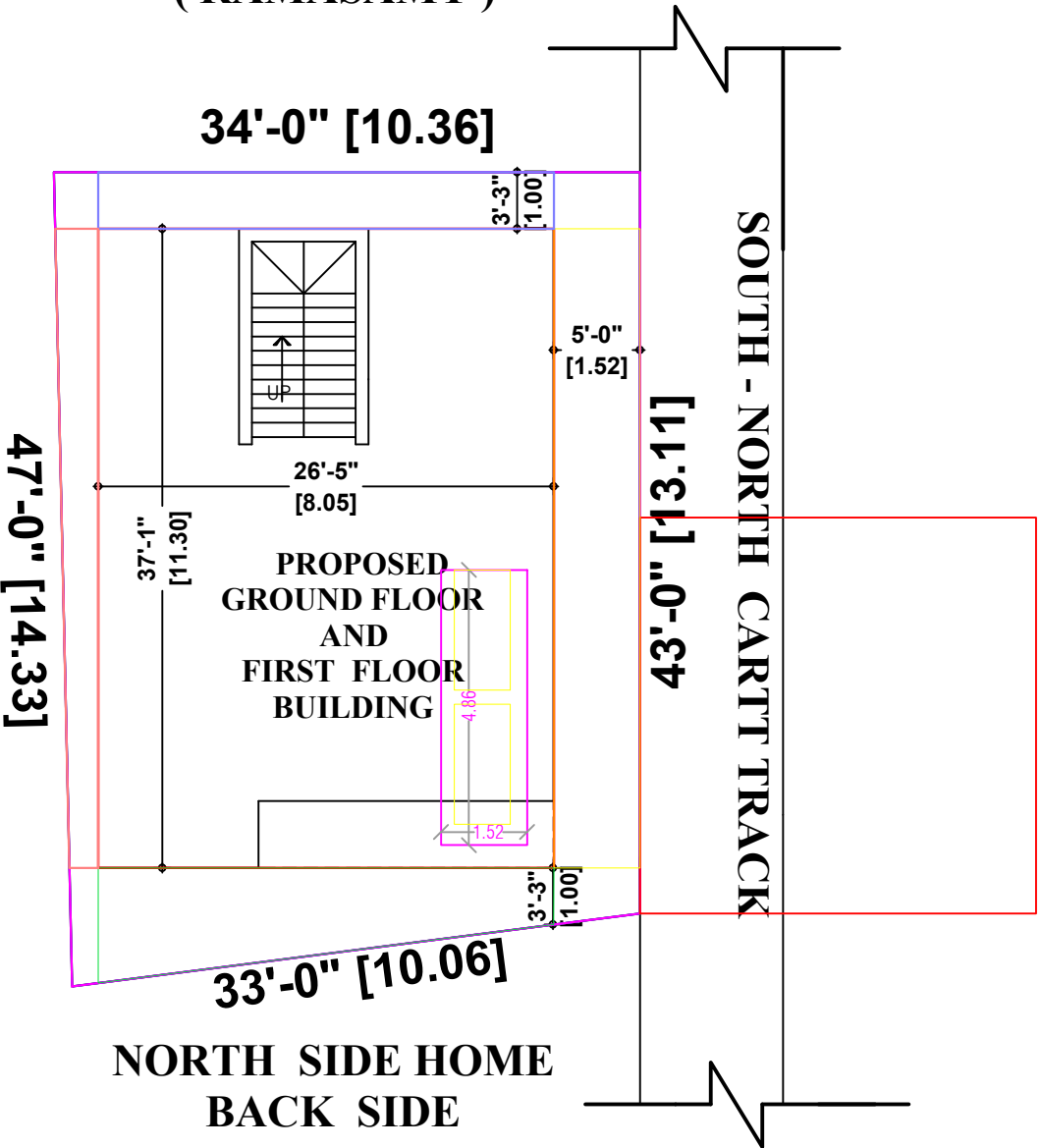
SITE PLAN
