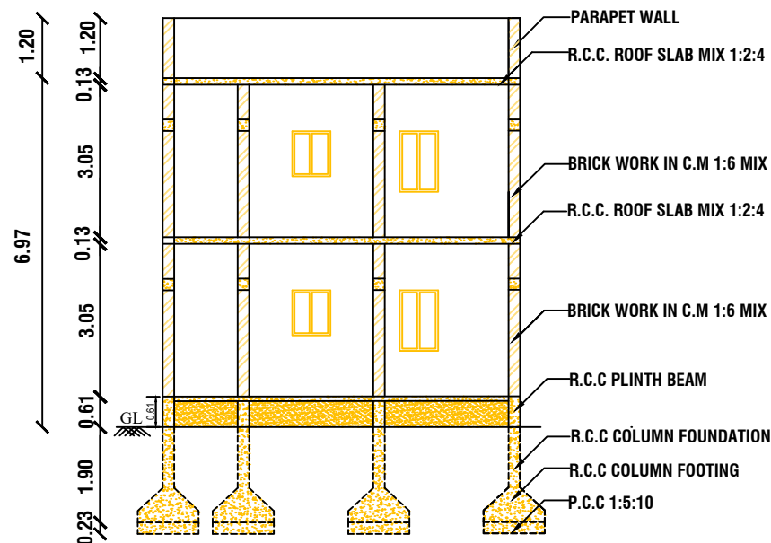
CROSS SECTION AT A-A
