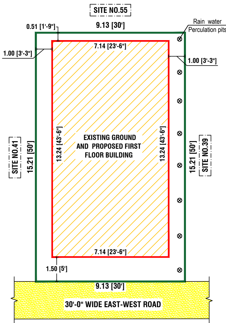
SITE PLAN
