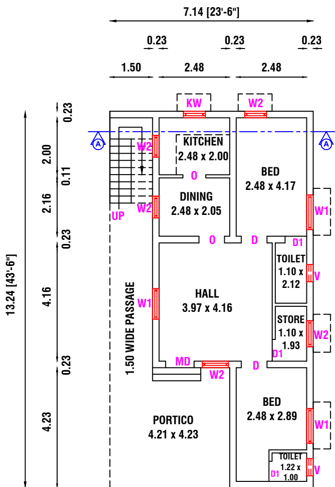
EXISTING GROUND
