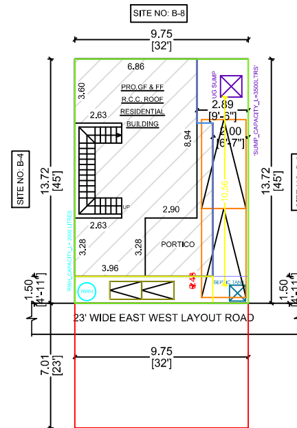
SITE PLAN
