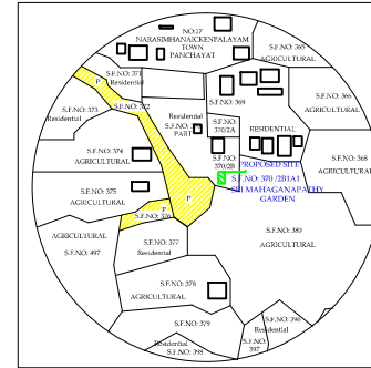
TOPO PLAN
