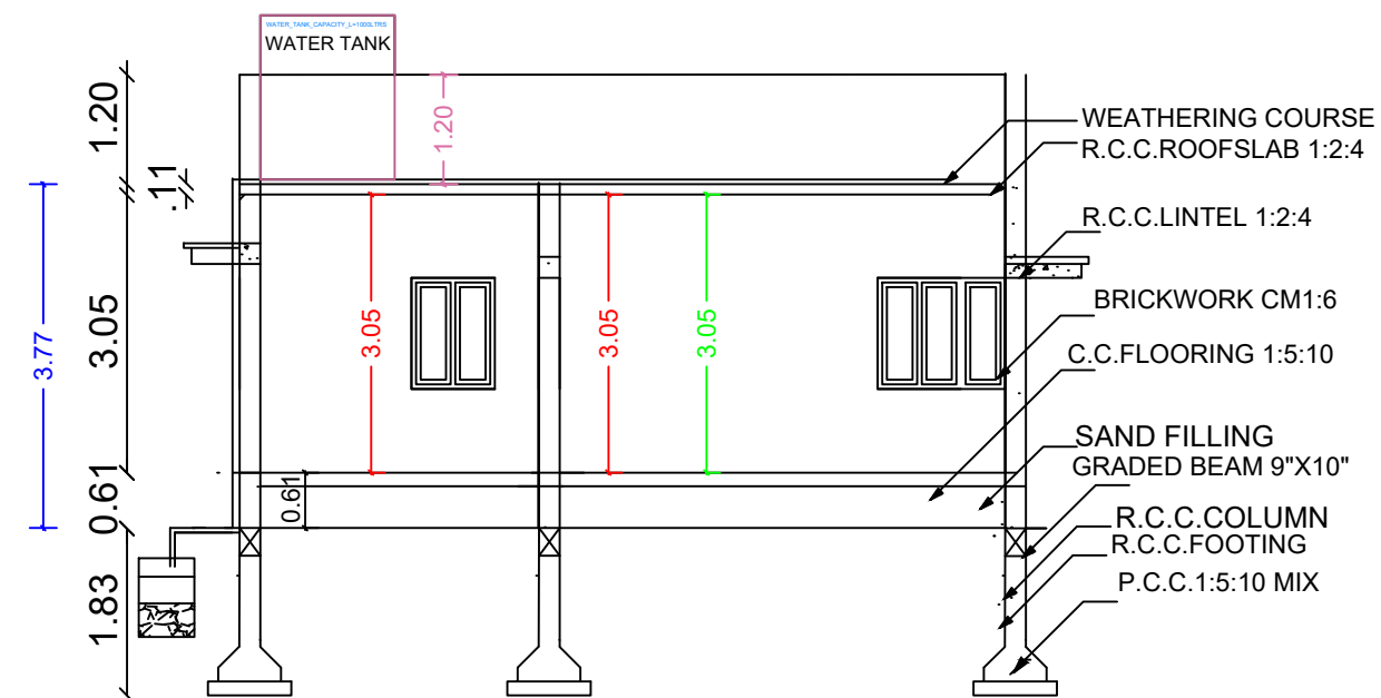
SECTION ON AB 9m NORTH SOUTH ROAD
