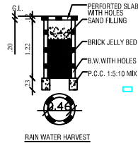
RAIN WATER HARVEST
