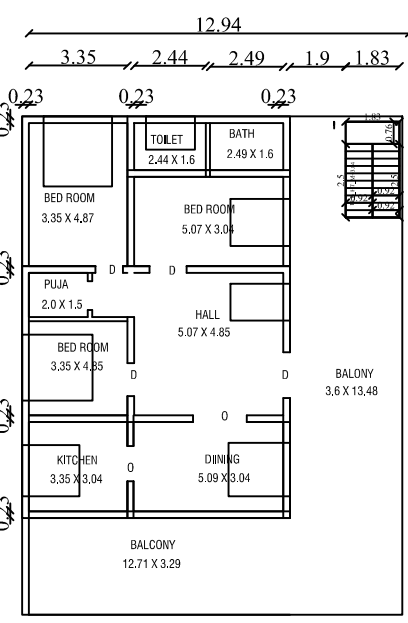
FIRST FLOOR BUILDING
