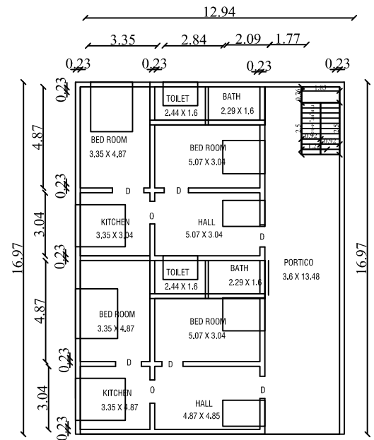
GROUND FLOOR BUILDING
