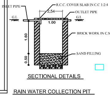
RAIN WATER COLLECTION PIT
