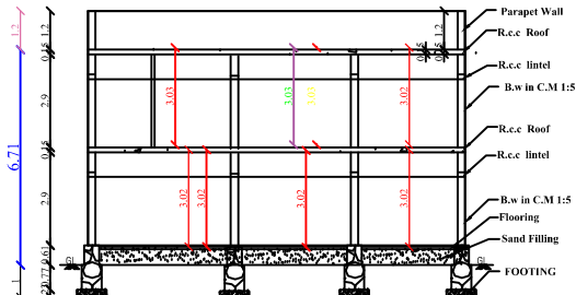
SECTION AB
