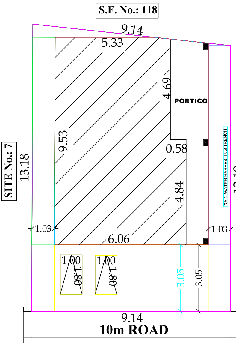
SITE PLAN
