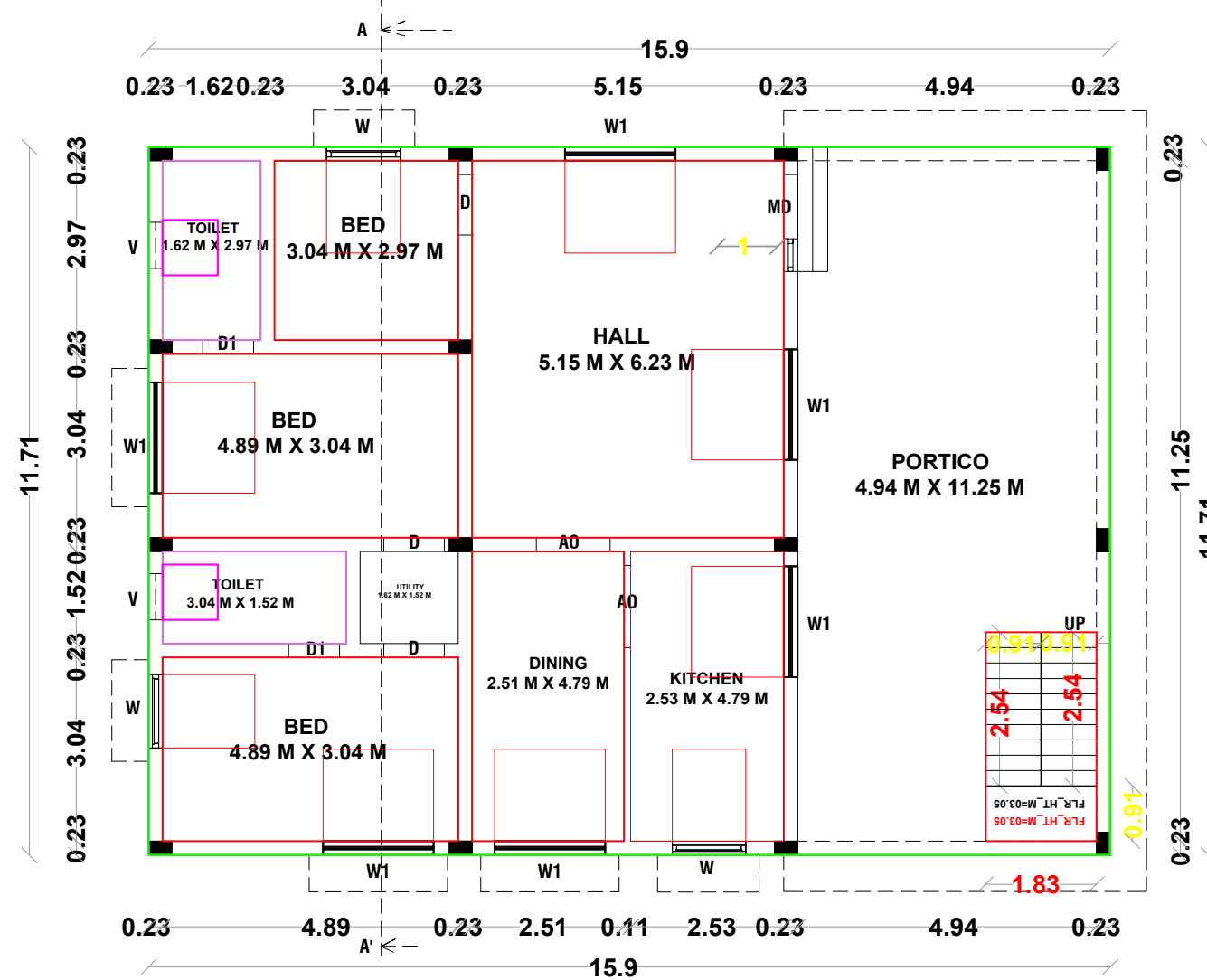
PROPOSED G.F PLAN
