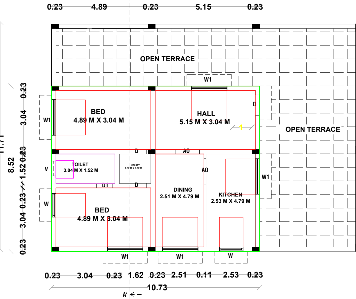
PROPOSED F.F. PLAN
