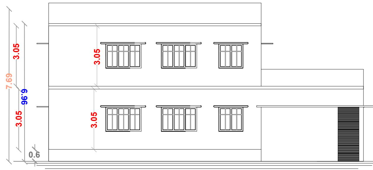
SOUTH SIDE VIEW
