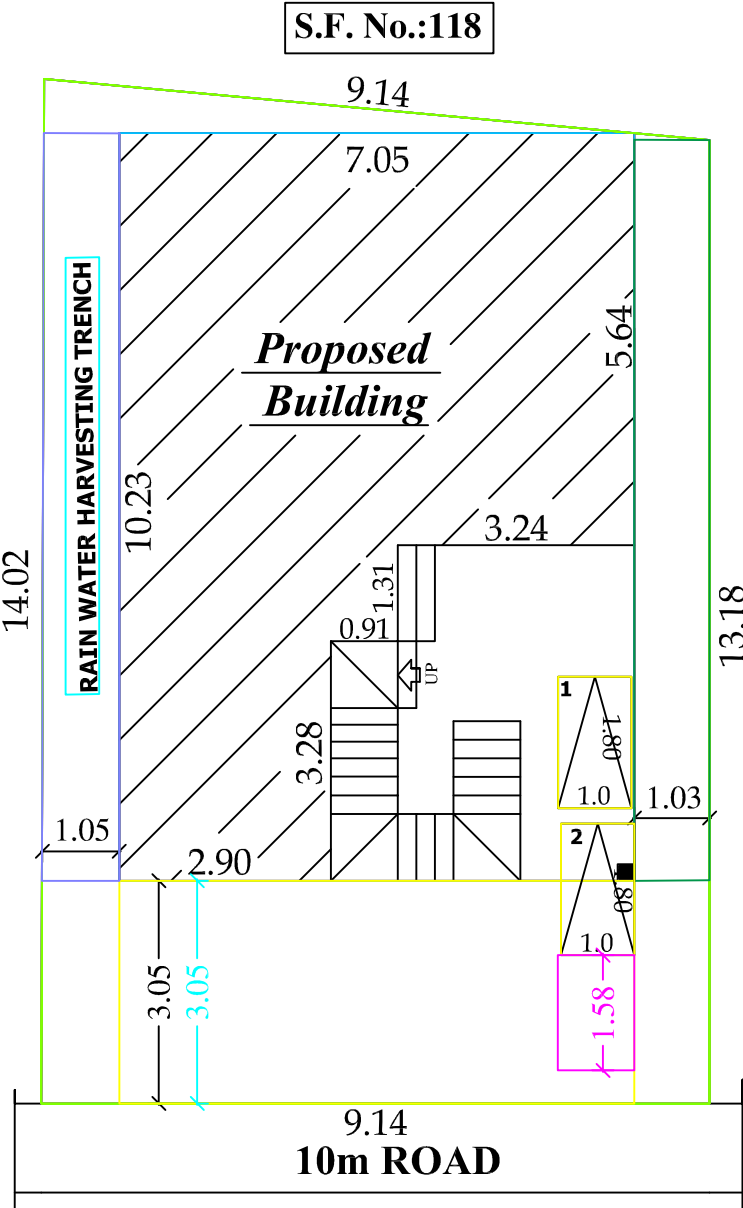
SITE PLAN
