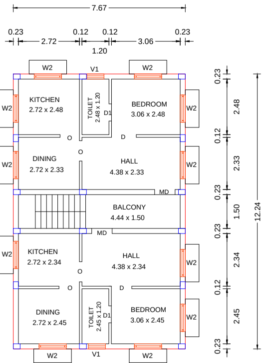
TYPICAL FLOOR PLAN (FIRST, SECOND, THIRD FLOOR)
