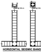
HORIZONTAL SEISMIC BANDS
