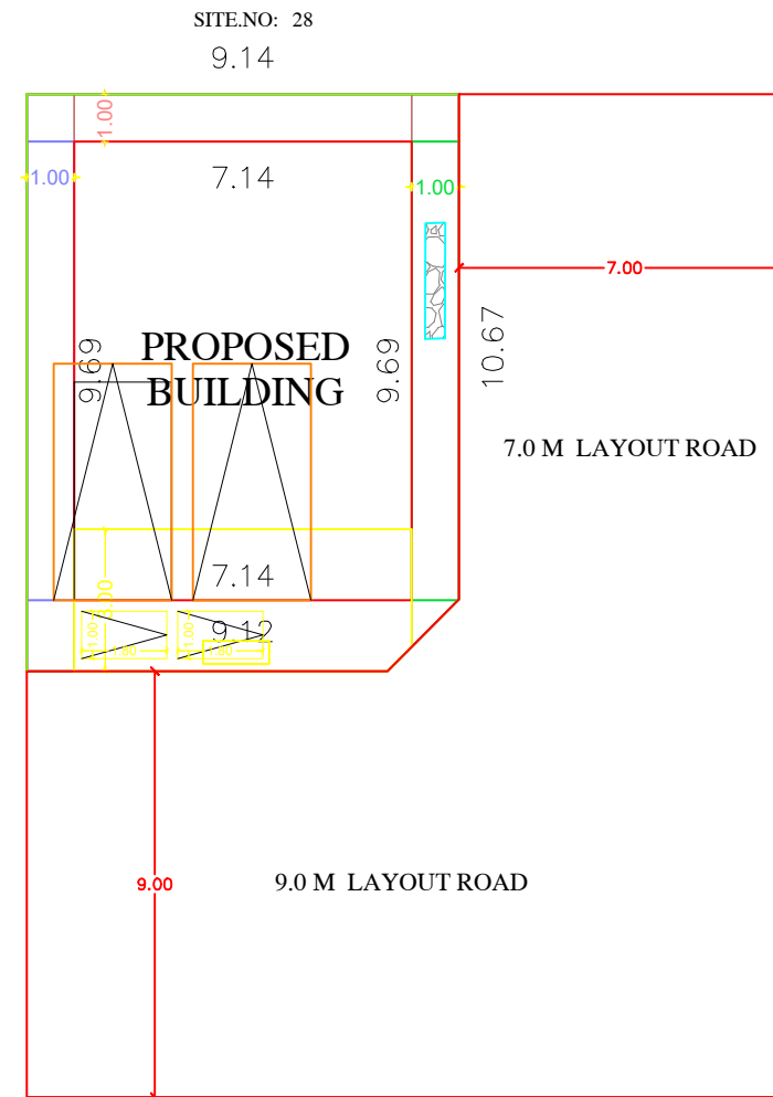
SITE PLAN
