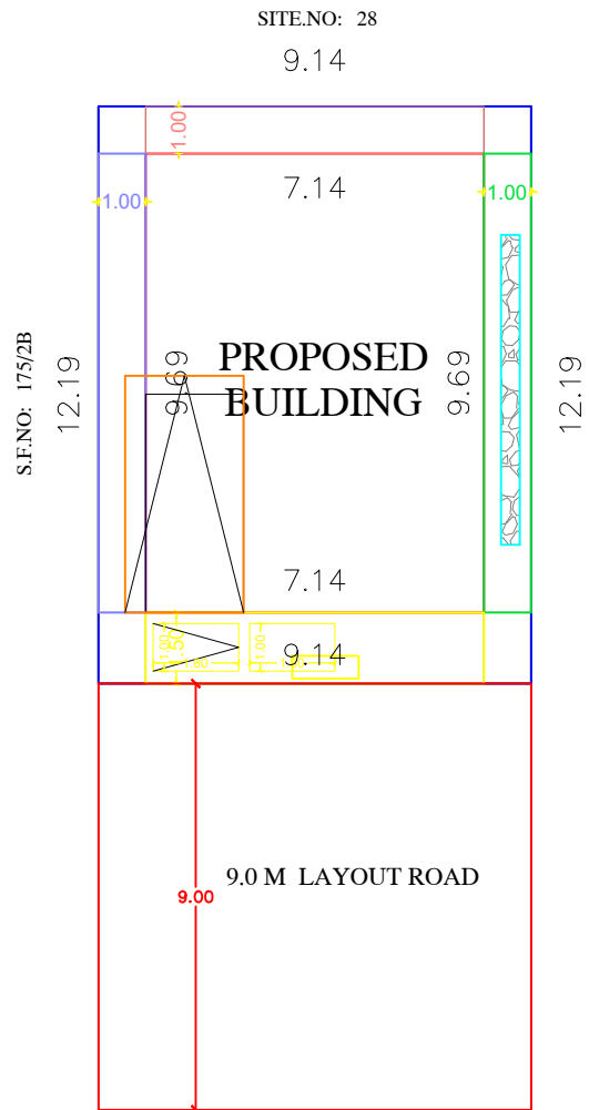
SITE PLAN
