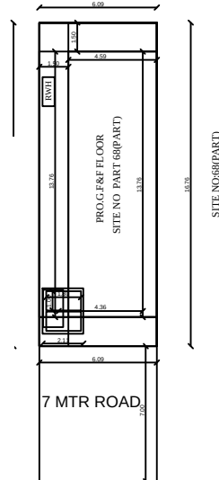
SITE PLAN
