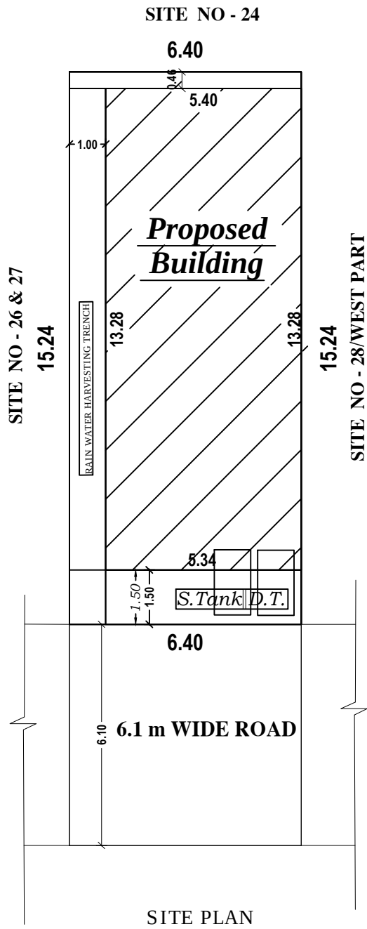
SITE PLAN
