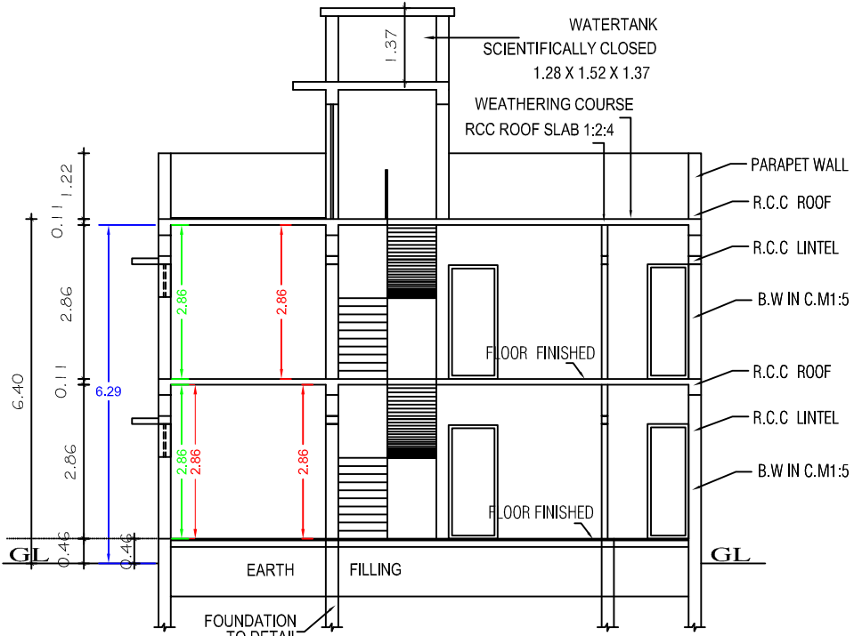
SECTION "A-B"
