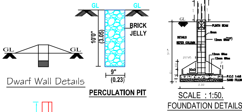
FOUNDATION DETAILS
