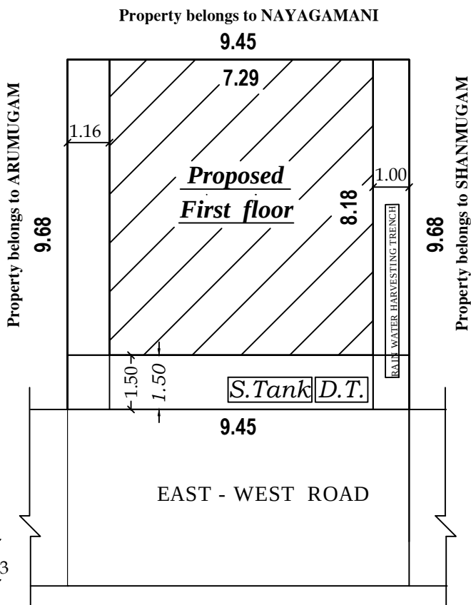
SITE PLAN
