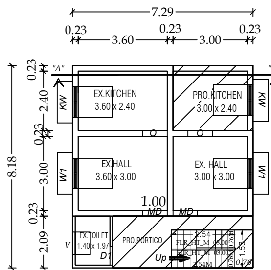
EX. & PRO. GROUND FLOOR PLAN
