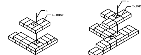
CORNER REINFORCEMENT IN CASE OF IN-BRICK MASONRY
