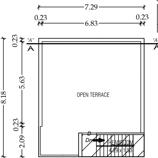
PRO. TERRACE FLOOR PLAN
