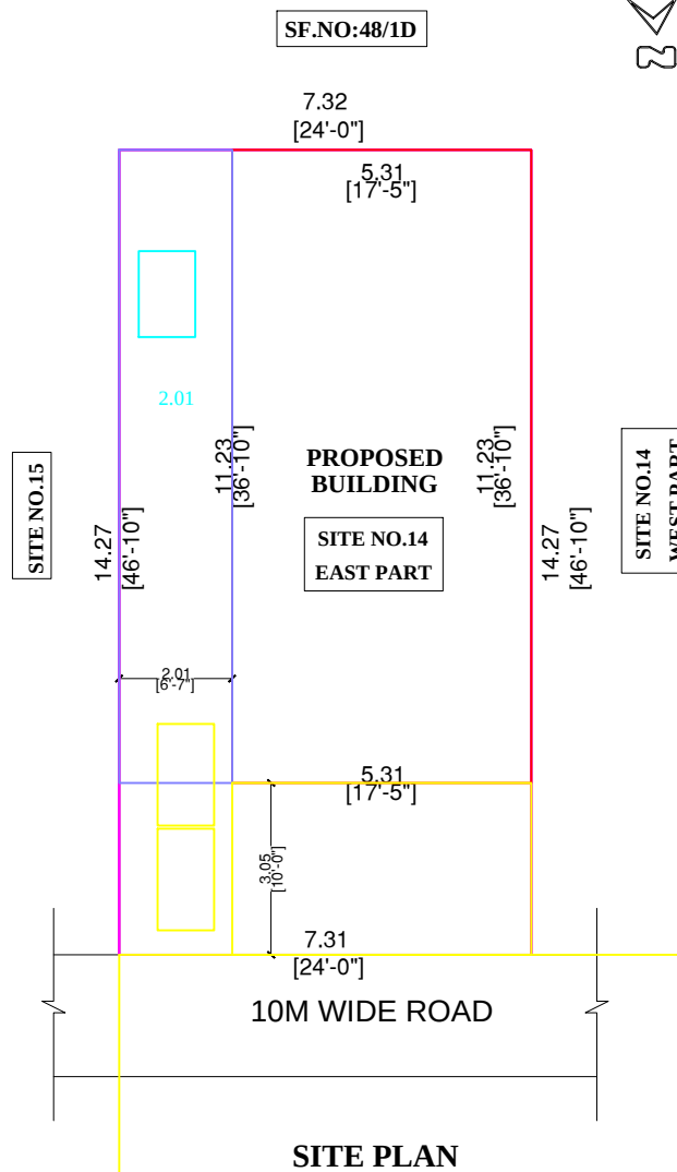
SITE PLAN
