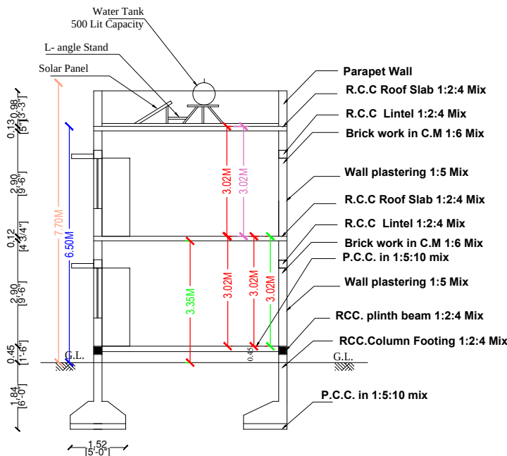
SECTION - AA
