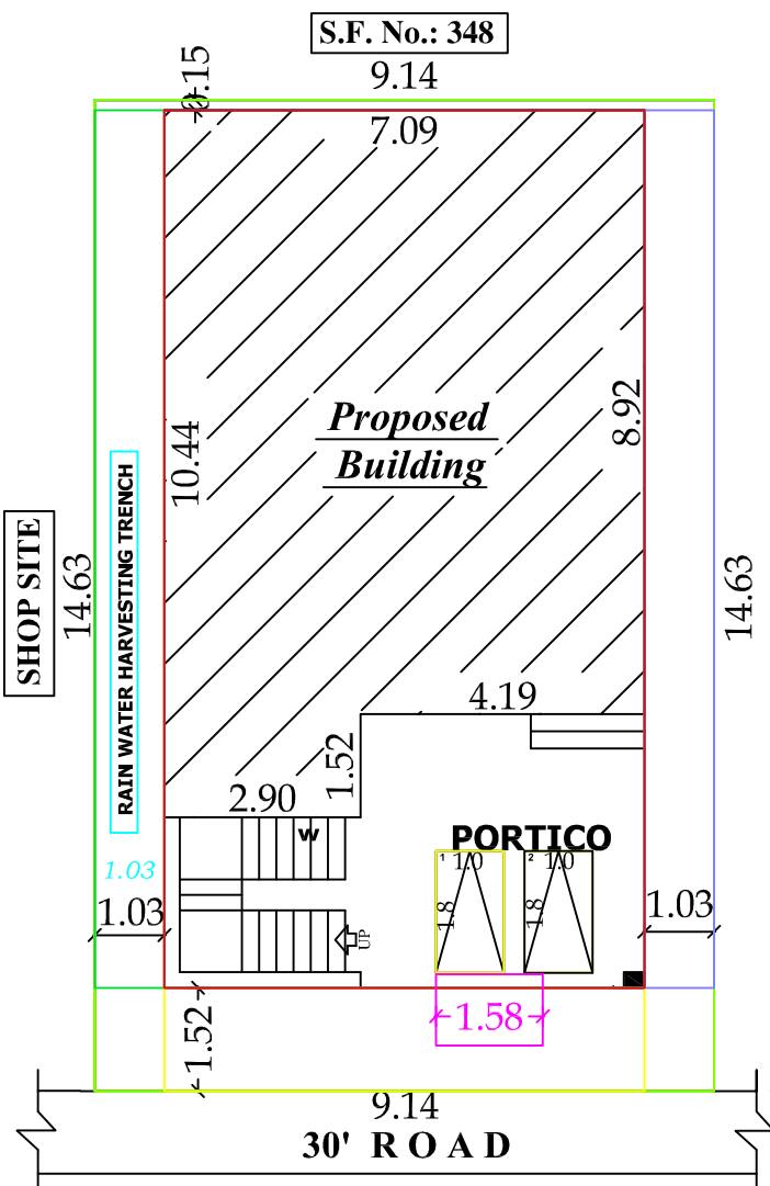
SITE PLAN
