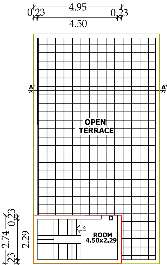
TERRACE FLOOR
