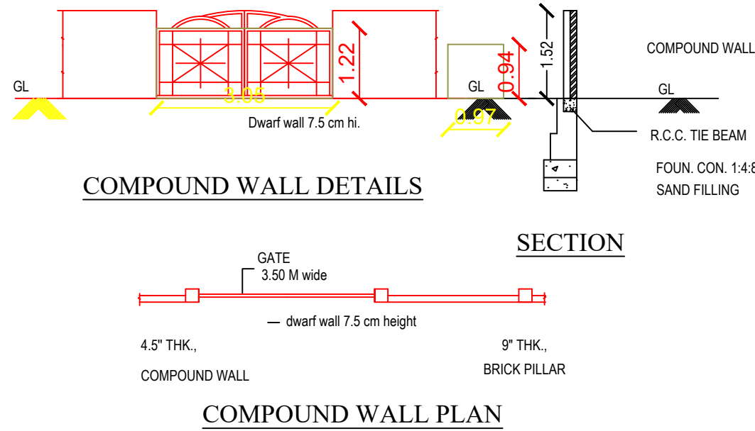
COMPOUND WALL PLAN
