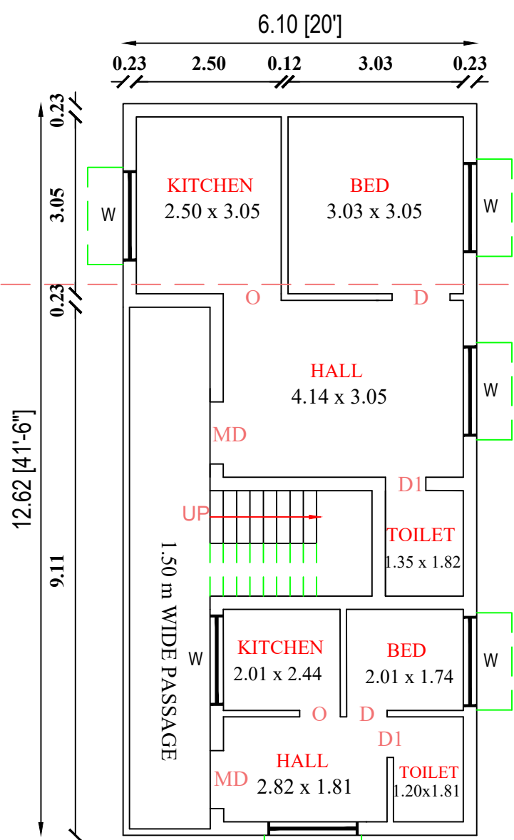
REVISED FIRST FLOOR PLAN
