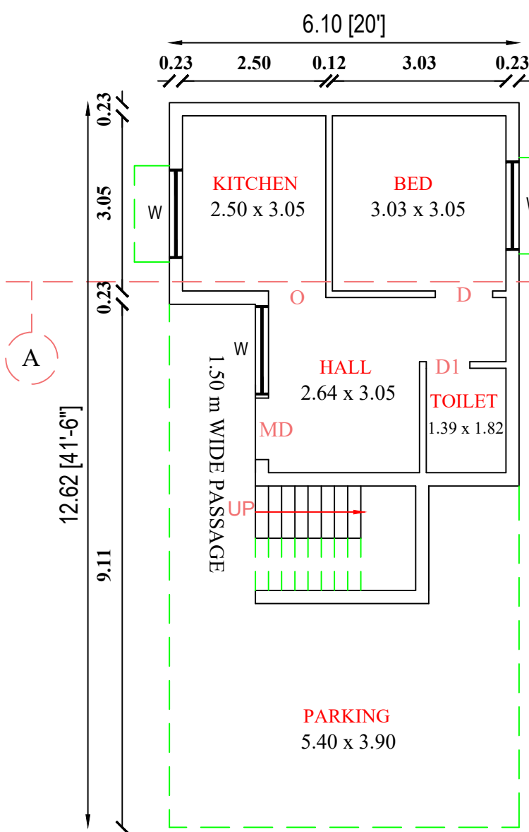
REVISED GROUND FLOOR PLAN
