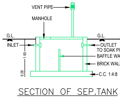
SECTION OF SEP.TANK
