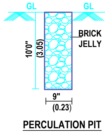
PERCOLATION PIT
