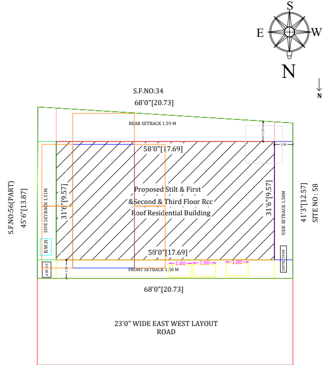
SITE PLAN
