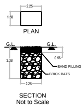
RAINWATER HARVEST PIT DETAILS
