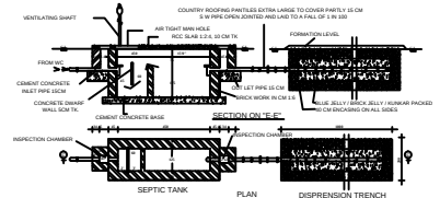
TYPE DESIGN FOR A SEPTIC TANK 10,000 LITRES CAPACITY (NOT TO SCALE)
