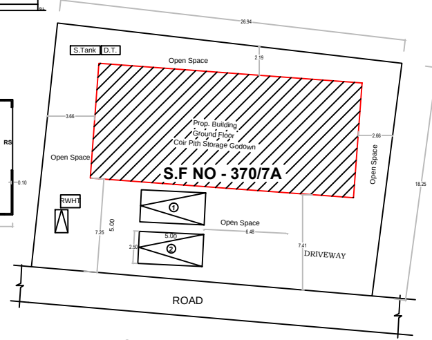
SITE PLAN
