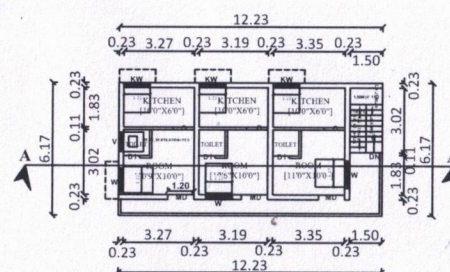
PROPOSED FIRST FLOOR
