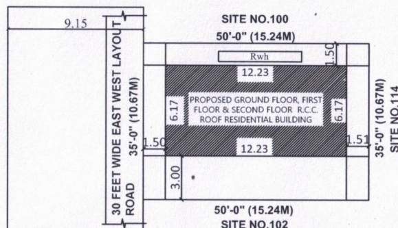
SITE PLAN
