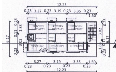
PROPOSED GROUND FLOOR
