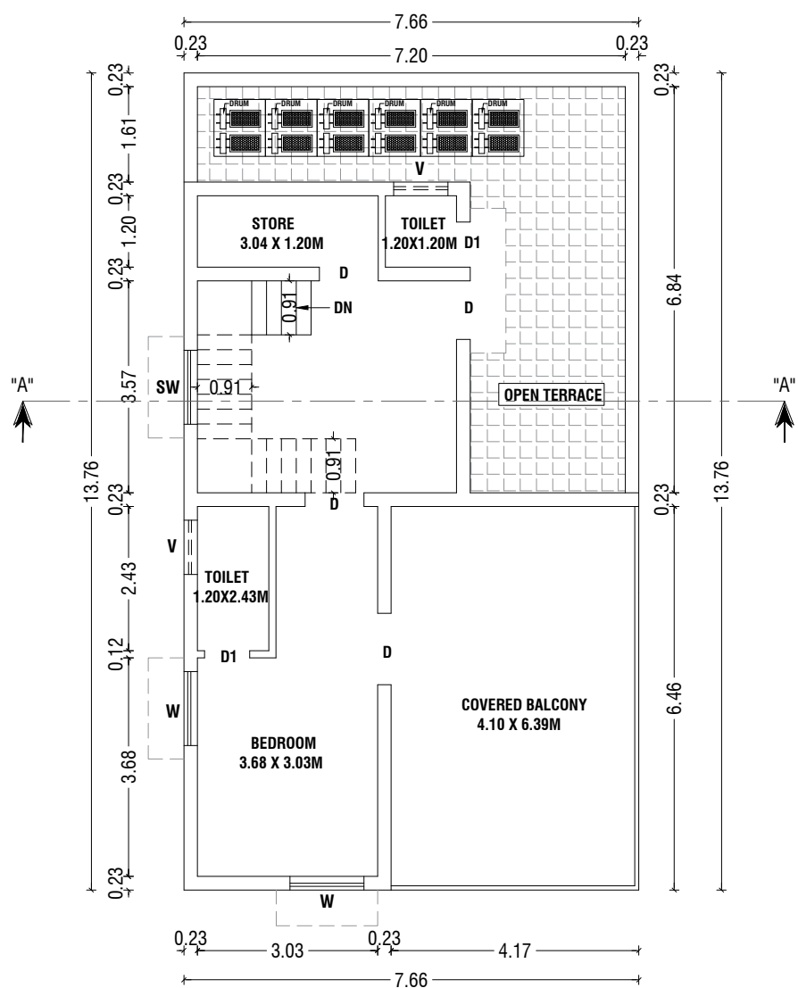
SECOND FLOOR
