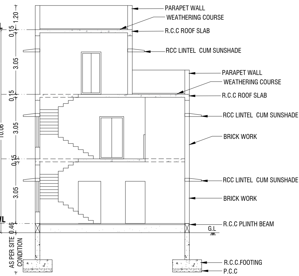
SECTION "AA" @ NORTH SIDE
