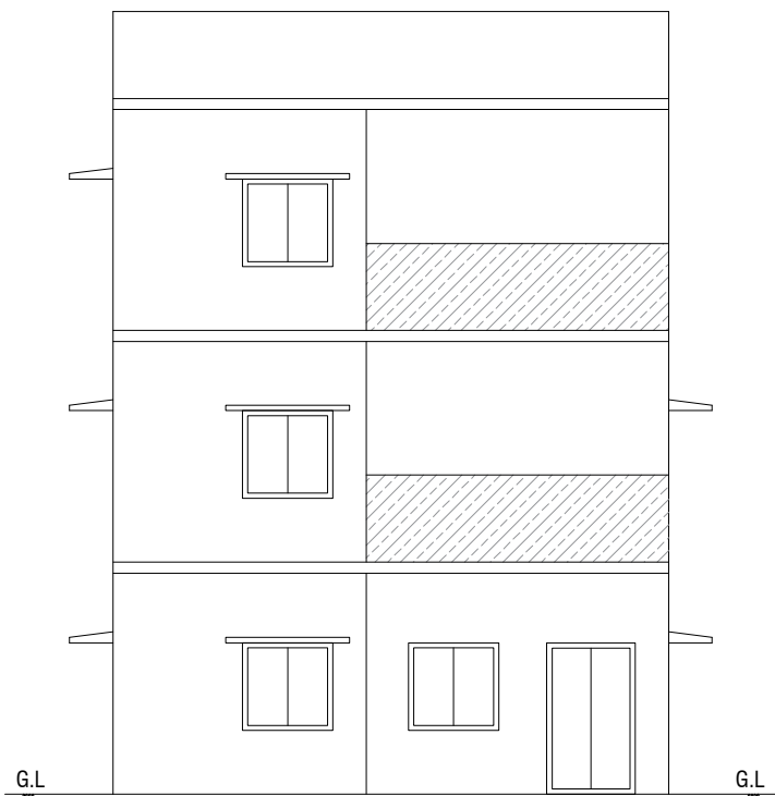
FRONT ELEVATION @ SOUTH SIDE
