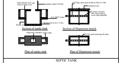
SEPTIC TANK
