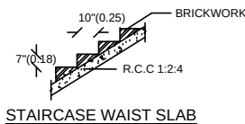
STAIRCASE WAIST SLAB
