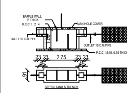
SEPTIC TANK & TRENCH
