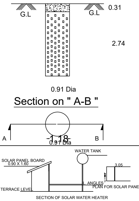
SECTION OF SOLAR WATER HEATER
