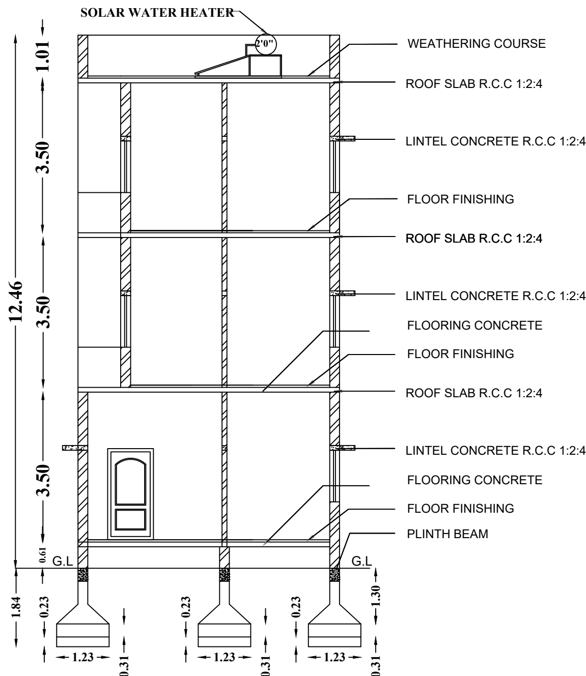
SECTION
